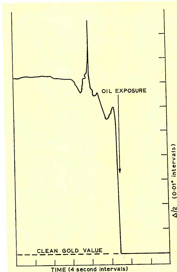
Fig. 4 Curve showing the very rapid adsorption of trichloroethylene from the vapour on to a clean gold surface
