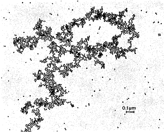
Electron micrograph of the finest gold suspension, with particle diameters of 160 Å
