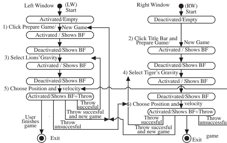
Figure 6. State diagram of the OO simulation of a basketball game
