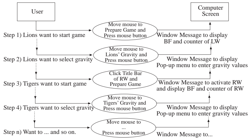
Figure 7. Functional model of the OO simulation of a basketball game
