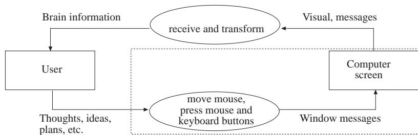
Figure 3. Counter-clockwise data-flow diagram with the system area and boundary as dotted line
