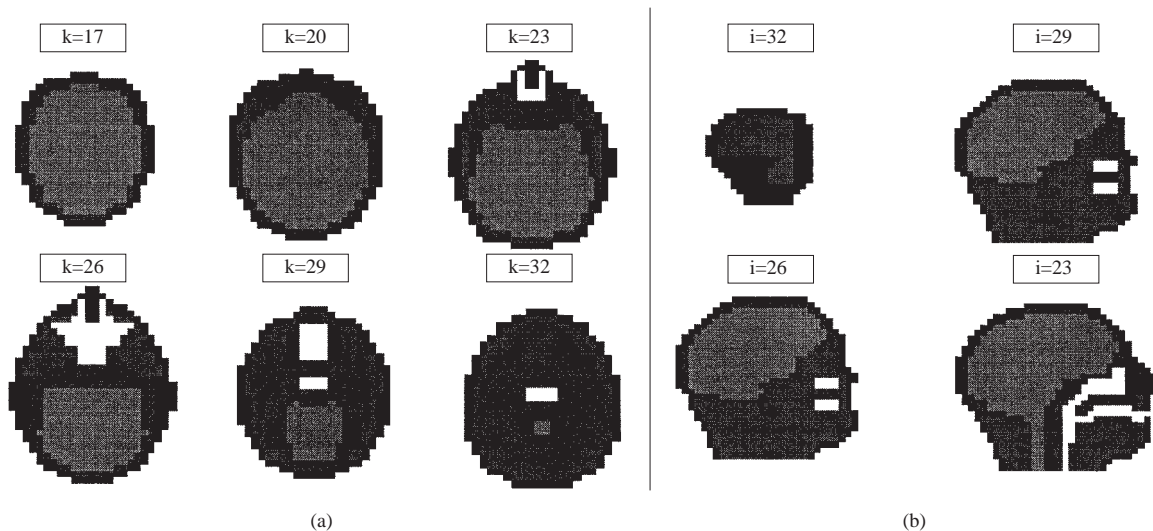
Figure 3. Horizontal ( k=17, 20, 23, 26, 29, 32 ) and vertical ( i=32, 29, 26, 23 ) slices of human head model showing different tissues.
