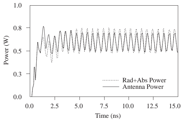
Figure 7. Time variations of instantaneous power calculated during FDTD simulation with both two dimensional closed surface and three dimensional volume integrations given in eq.s(17)-(19).
