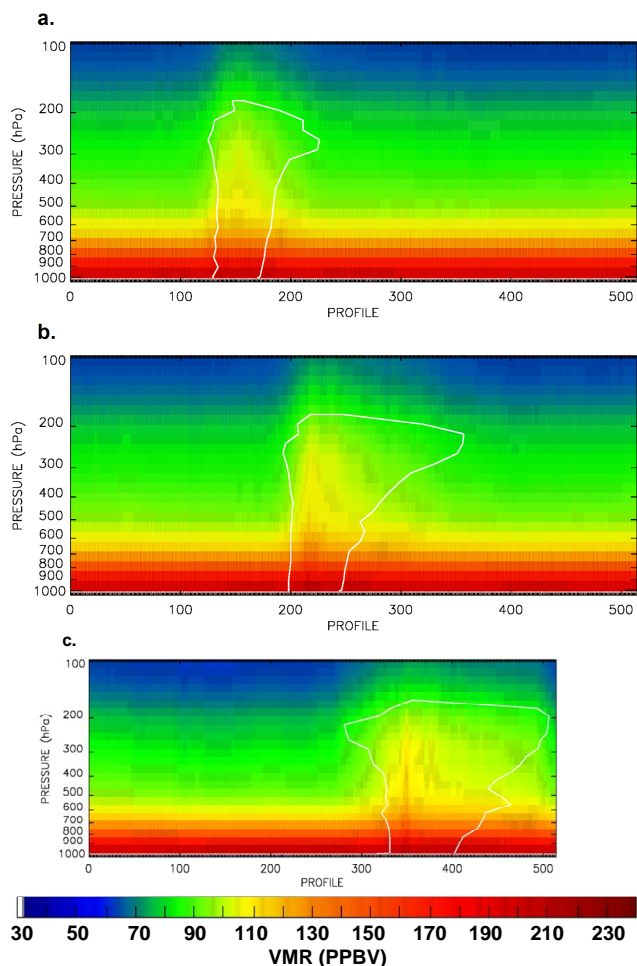
Fig. 15. Synthetic TES retrievals (ppbv) at (a) 180 min, (b) 300 min, and (c) 480 min. The white outline in the figure is the region of clouds associated with the storm system. TES retrievals in regions below and within this area are interpreted as being unrealistic because of the “clear-sky” averaging kernel used for the profiles.
