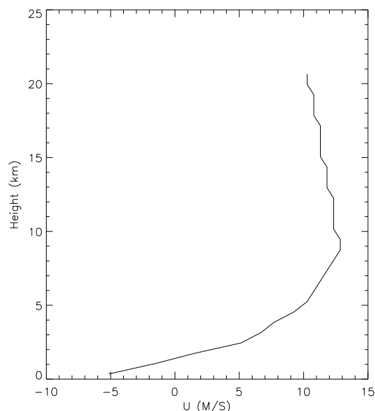
Fig. 5. The vertical wind profile used in the squall line simulation.
