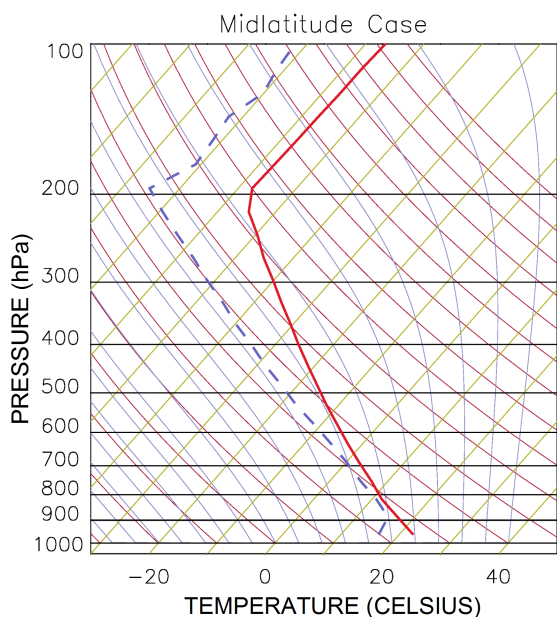
Fig. 3. Thermodynamic sounding of the pre-squall line environment used for the squall line simulation in this study. The solid red line denotes temperature, while the dashed blue line shows dew point temperature. The sounding is similar to that at Lincoln, IL at 00:00 UTC 13 March 2006 during INTEX-B.
