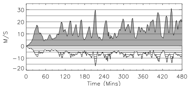
Fig. 6. Time-series of maximum updraft speed ( W , positive values) and maximum downdraft speed ( W , negative values) in \text{m s}^{-1} during the entire 8-h squall line simulation period.
