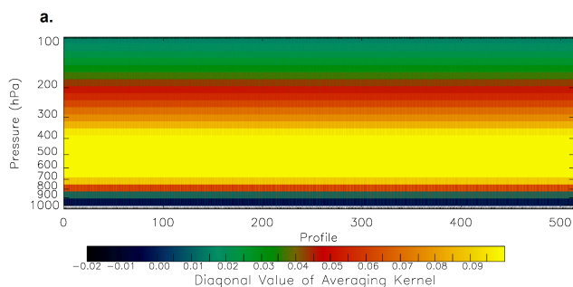
Fig. 13. Clear sky averaging kernel diagonal used in the TES retrievals from profile 14 of RUNID 3443 on 13 March 2006 (see location in Fig. 2a) that was applied to all horizontal grid points in the 2-D GCE model domain
