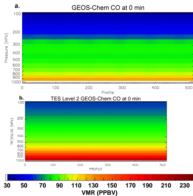
Fig. 14. (a) Initial CO concentration (ppbv) used in the GCE simulation, (b) Synthetic TES retrievals of the initial CO concentration (ppbv).
