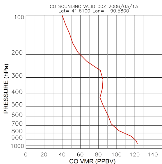
Fig. 4. CO profile (ppbv) from the GEOS-Chem model used as the background concentration in the GCE for the squall line simulation. The profile is valid at 00:00 UTC 13 March 2006 at 41.61° N, 90.58° W.
