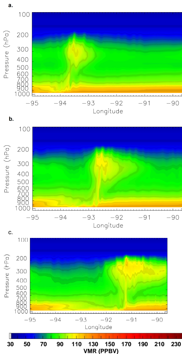
Fig. 10. Simulated CO concentration (ppbv) after (a) 180 min, (b) 310 min, and (c) 480 min.
