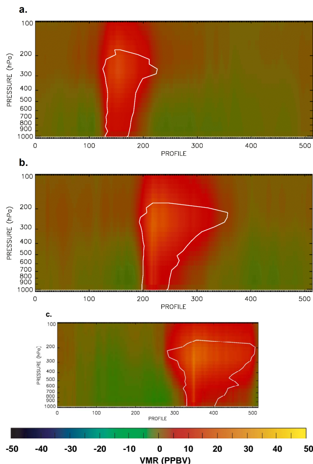
Fig. 16. Plots of the difference (ppbv) between synthetic TES CO retrievals and the initial CO concentration (as seen by TES) at (a) 180 min, (b) 300 min, and (c) 480 min. The white outline is the region of the storm clouds, as in Fig. 15.
