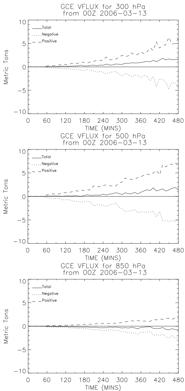
Fig. 11. Time series of vertical CO mass flux (t per 10 min period) at (a) 300 hPa (b) 500 hPa, and (c) 850 hPa during the entire model simulation period.
