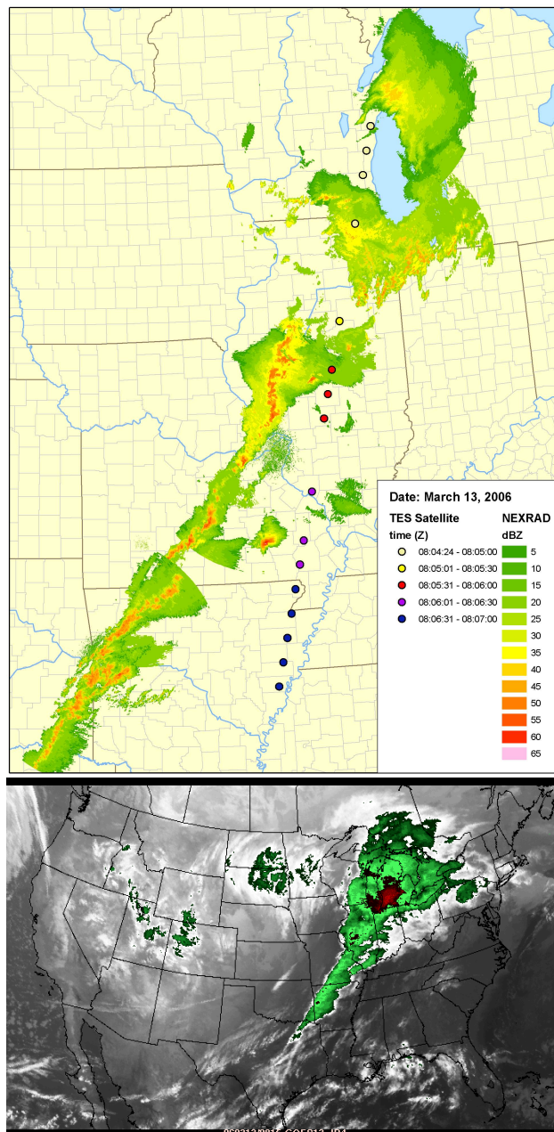
Fig. 2. (a) Radar reflectivity of the squall line (dBZ) at 08:04 UTC 13 March 2006, along with TES retrieval locations. The reflectivities are a composite from individual National Weather Service WSR-88D (NEXRAD) radars in the area. TES moves from NE (location 0) to SW (location 15), crossing the squall line near Lincoln, IL. The TES footprints are color-coded to show the time of each retrieval. The averaging kernel profile at site 14 (second from the south) was used to make our synthetic TES retrievals. Since the GCE is run in the x-z plane, its axis along the length of the squall line is arbitrary. (b) GOES-12 enhanced infrared satellite image for 08:15 UTC 13 March 2006.
