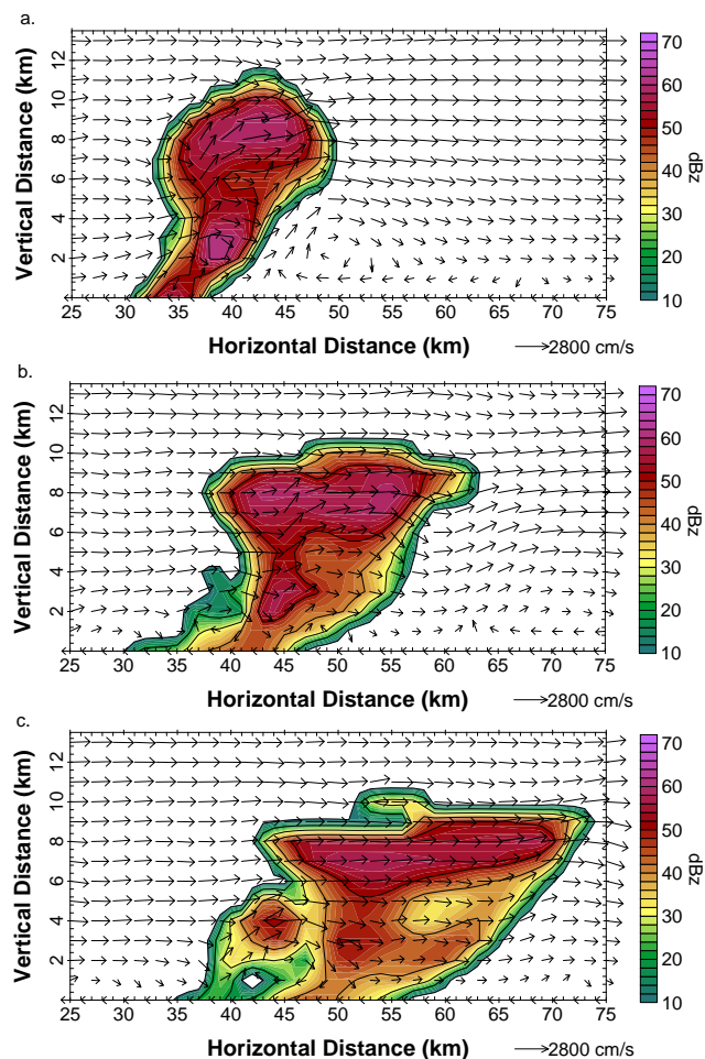
Fig. 7. U- W wind vectors and reflectivities (dBZ) at (a) 40 min, (b) 50 min, and (c) 60 min into the simulation. The longest arrow represents the maximum wind of (a) 27 \text{ m s}^{-1} , (b) 24 \text{ m s}^{-1} , and (c) 23 \text{ m s}^{-1} .
