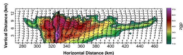
Fig. 9. Reflectivity pattern (dBZ) at the end of the 8 h simulation.
