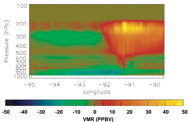
Fig. 12. Change in CO concentration (ppbv) during the overall 8 h simulation.
