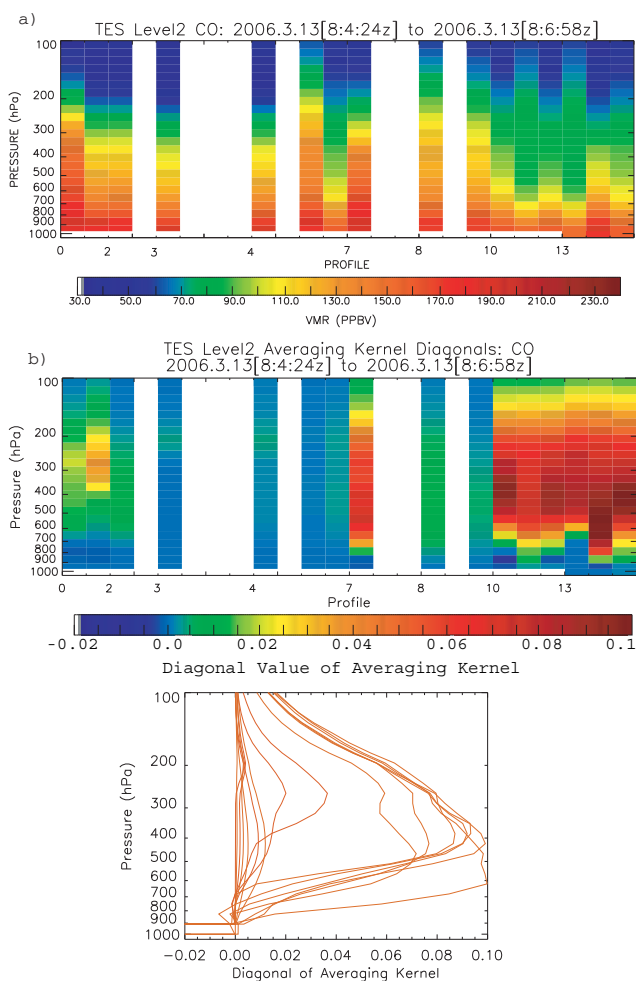
Fig. 17. (a) Observed TES CO retrievals (ppbv) for RUNID 3443 at 08:04 UTC 13 March 2006 for profiles 0–15, (b) TES averaging kernel diagonals for RUNID 3443 and profiles 0–15. Profiles 0 (15) are the northern most (southern most) sites in Fig. 2a.
