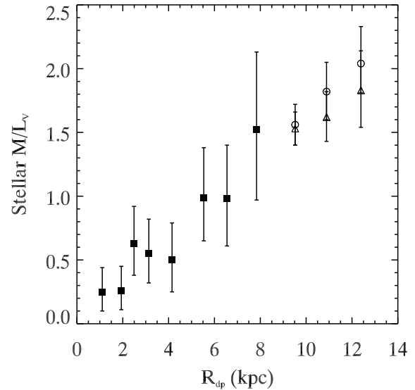
Fig. 1. V-band stellar mass-to-light ratio in M33.
