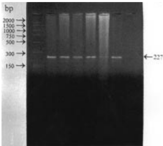
Figure 1. Agarose gel electrophoresis analysis of PCR-amplified genomic DNA by using Apo E primers (see methods section). The size of the amplified fragment is 227 bp. Lanes show the amplified fragment using 1 µg genomic DNA from blood.
