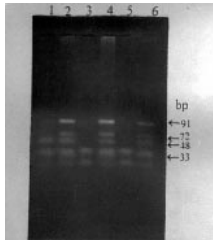
Figure 2. Gel electrophoresis analysis of CfoI digestion of PCR product. The 227 bp PCR products were cut by CfoI (see methods section). Lanes 2,4,6: Apo E genotype is \epsilon 4/\epsilon 3 . Lanes 3,5: Apo E genotype is \epsilon 4/\epsilon 4 . Lane 1: Apo E genotype is \epsilon 3/\epsilon 3
