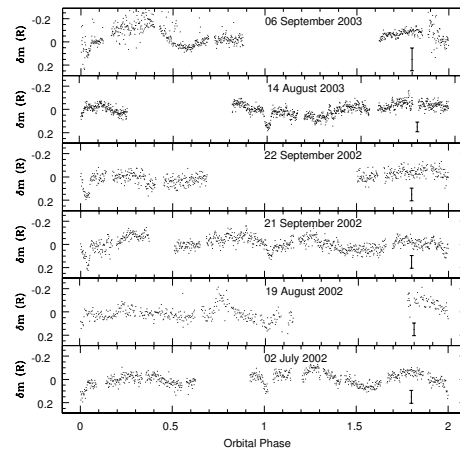
Fig. 1. Light curves at the six different epochs. The mean 3\text{-}\sigma errorbar for each epoch is included in each panel.
