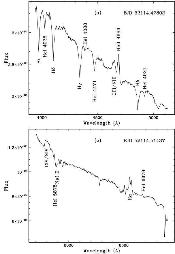
Fig. 1. Spectra around the outburst maximum. We can see emission lines of H\alpha , He II 4686, C III/N III around 4630, and C IV/N IV around 5800, and absorption lines of other Balmer lines, He I, and Na I D on a blue continuum.
