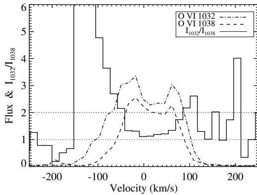
Fig. 3. E1 MDRS spectrum: O VI line fluxes and ratio between them.
