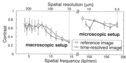
Fig. 4 Transverse imaging resolution of the proposed system. Contrast curve of the time-resolved image is compared with that of the reference image without OKG with regard to spatial frequency. Line is a guide for the eye.
