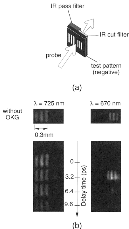
Fig. 6 Time-resolved spectroscopic imaging of colored transparent object. (a) Schematic view of sample and (b) temporal evolution of the two images obtained with the femtosecond amplifying OKG at 725 and 670 nm.
