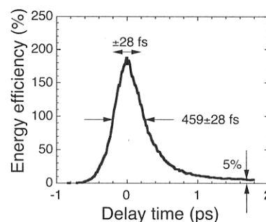
Fig. 3 Temporal behavior of femtosecond amplifying OKG signal.
