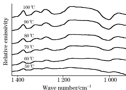
Fig. 3 The temperature dependence of emission FTIR spectra of PEO 10 -LiClO 4 /5% m SBA-15
