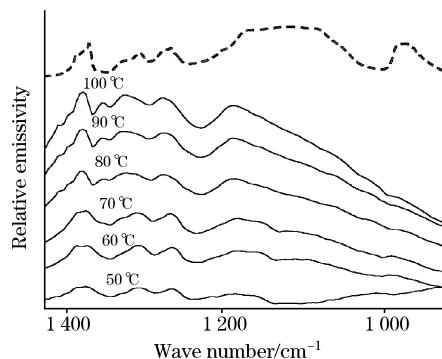
Fig. 2 Temperature dependence of emission FTIR spectra of PEO 10 -LiClO 4 , the dot line is transmission spectrum at room temperature
