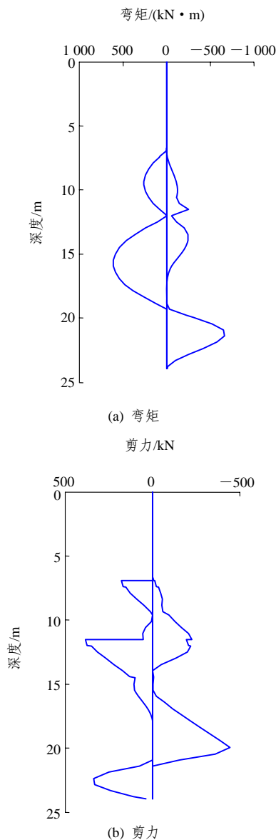
图2 支护结构弯矩及剪力包络图 Fig.2 Moment and shear force distribution
