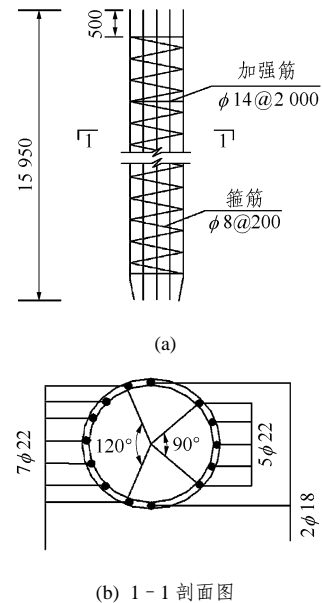
图4 护坡桩配筋图 Fig.4 Reinforcement of pile
