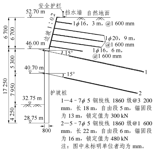
图3 基坑支护设计详图 Fig.3 Supporting design of the pit
