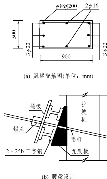
图5 冠梁及腰梁设计图 Fig.5 Design of cap beam and wale
