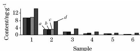
Fig. 1 Standard values of the certified reference materials and the results of determination by ICP-MS (with/without ORS mode)
