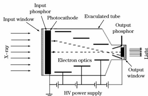
Fig. 2 The scheme of the conventional X-ray image intensifier
