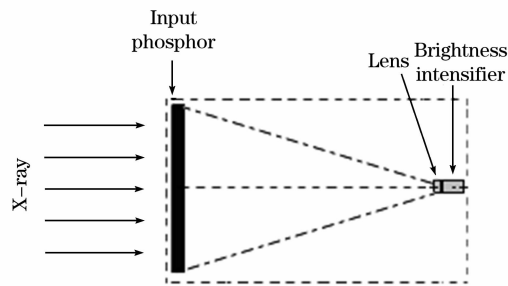
Fig. 3 The scheme of the novel X-ray image intensifier
