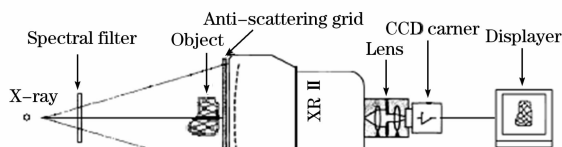
Fig. 1 The schematic diagram of the X-ray imaging system
