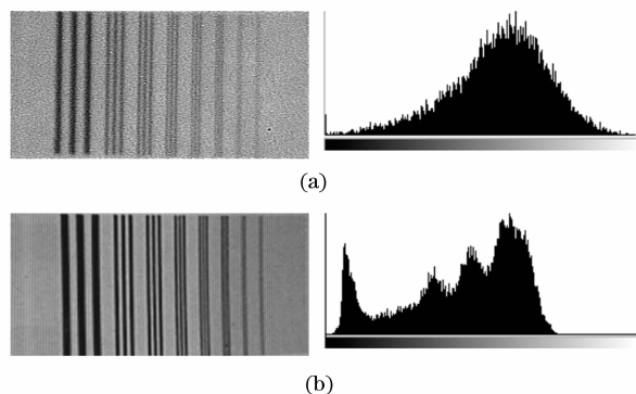
Fig. 4 The images produced by two kinds of X-ray image intensifier
