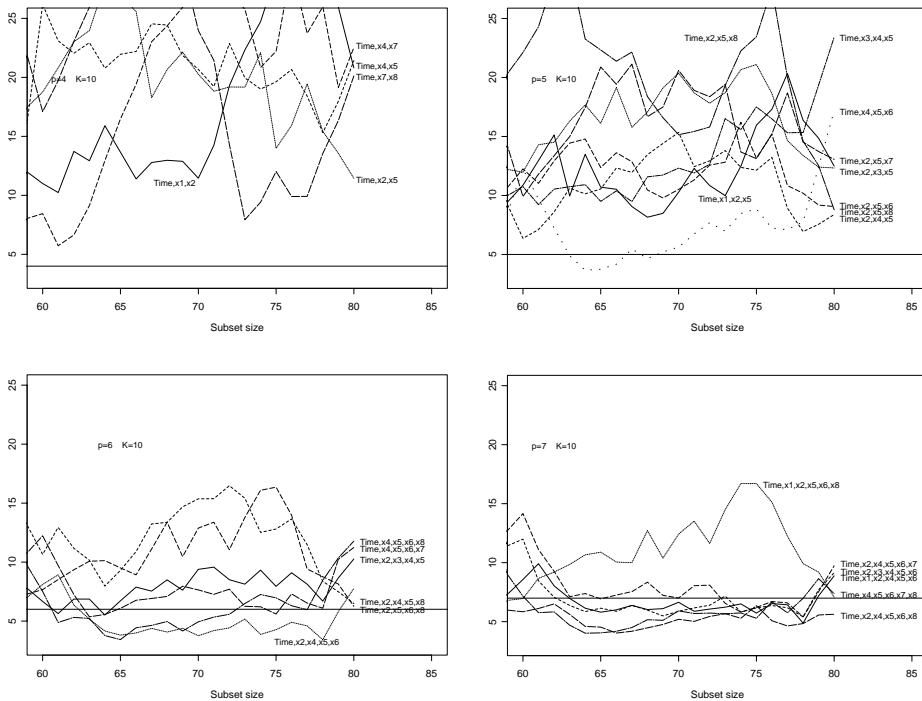
Figure 4. Ozone data: forward plots of C_p(m) when p = 4, 5, 6 and 7 . The last two observations to enter the subset have a clear effect on model choice.
