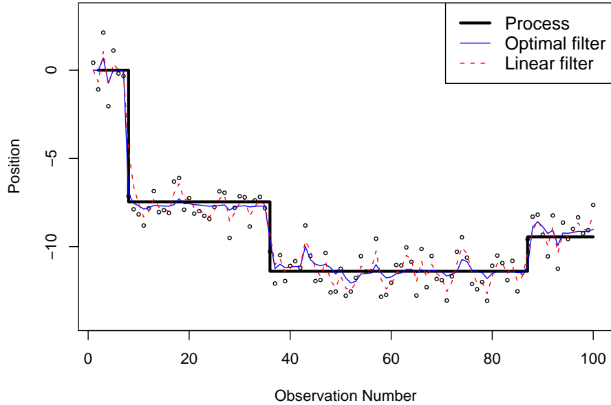
Figure 1: optimal non-linear and linear filters
