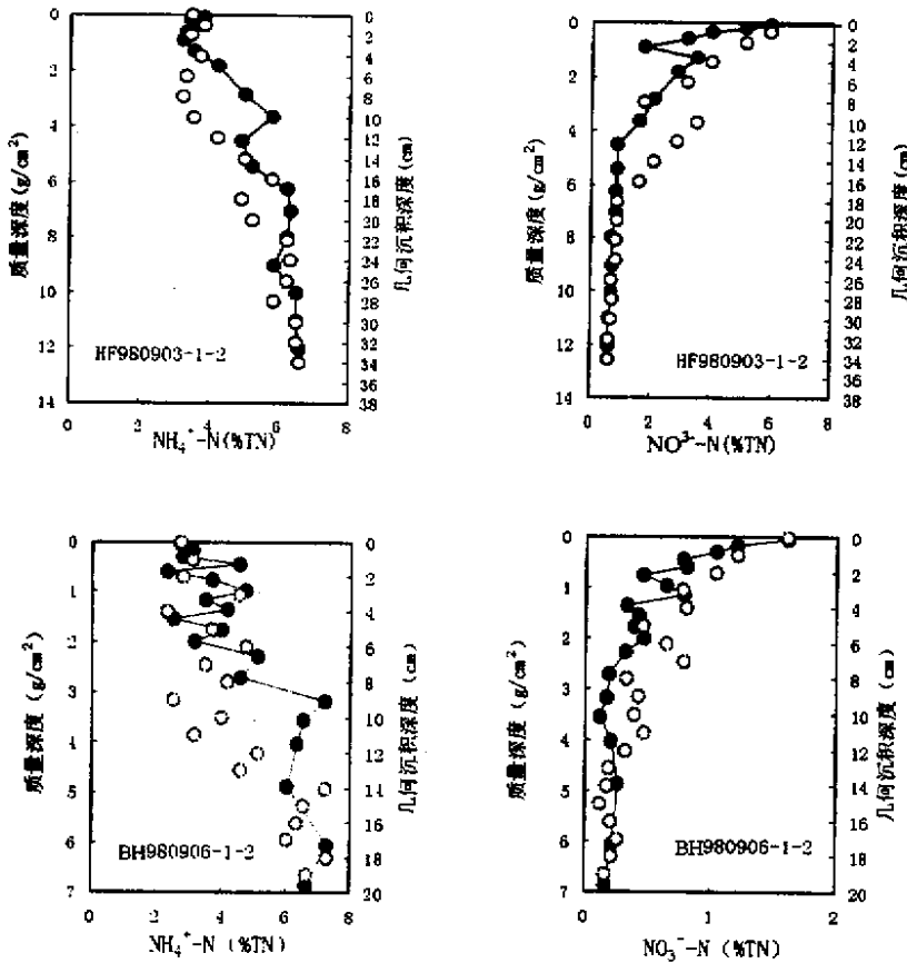
图 4 红枫湖、百花湖沉积物交换性无机氮相对于全氮百分比的剖面分布 Fig.4 Profiles of concentration percentage of exchangeable nitrogen in the sediment cores of Lake Hongfeng and Baihua
