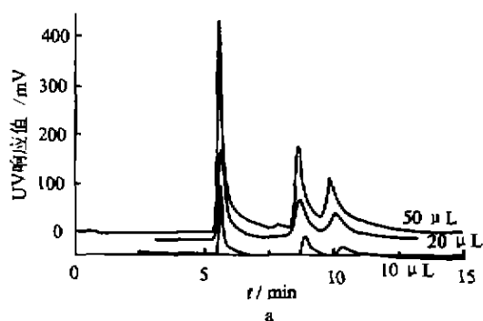
Fig. 2 SFC Chromatogram of hydrolyzate of egb extract conditions: YWG-SiO 2 10 \mu\text{m} column, 25 MPa, 50 ^{\circ}\text{C} mobile phase: CO 2 -ethanol (90:10 V/V) with \varphi(\text{H}_3\text{PO}_4) = 0.5\% in ethanol flowrate: 3.0 mL/min
