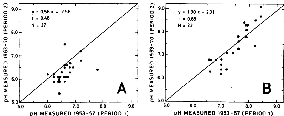
Fig. 5. Hydrogen-ion concentration (pH) in lakes in south-eastern Norway. x-axis: values measured in period 1, y-axis: values measured in the same lakes in period 2. Solid lines: positions for dots if no change from period 1 to period 2. (A): low-total-hardness lakes ( 0-1^{\circ} dH) [ 1^{\circ} dH = 10 \text{ mg } \text{CaO} \llbracket / \rrbracket ]. (B): High-total-hardness lakes ( > 1^{\circ} dH).
