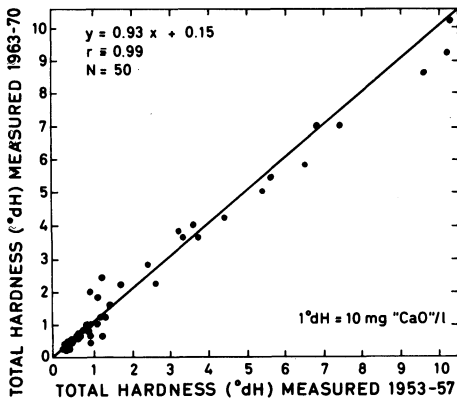
Fig. 4. Total hardness in 50 lakes in south-eastern Norway. x-axis: values measured in period 1 (1953-57), y-axis: values measured in the same lakes in period 2 (1963-70). Solid line: position for dots if no change from period 1 to period 2.
