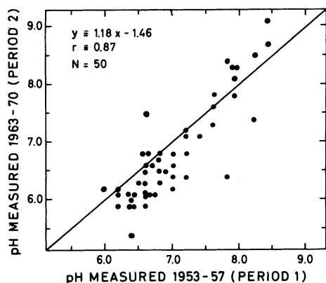
Fig. 3. Hydrogen-ion concentration (pH) in 50 lakes in south-eastern Norway. x-axis: values measured in period 1, y-axis: values measured in the same lakes in period 2. Solid line: position for dots if no change from period 1 to period 2.
