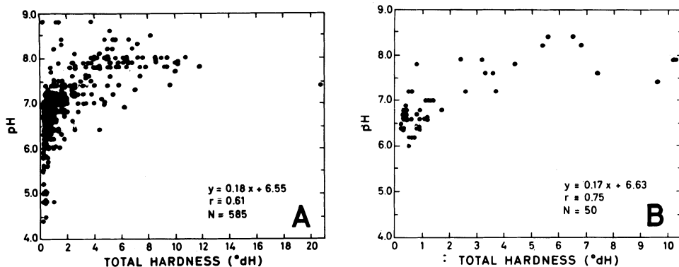
Fig. 2. (A): Total hardness and hydrogen-ion concentration (pH) in 585 lakes investigated 1953-70 in south-eastern Norway. (B): Same as in (A), indicating values for 50 lakes which were investigated twice. Values in (B) are from the first investigation period (1953-57). Note stretched scale for total hardness in (B):
