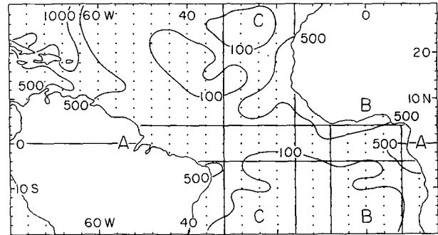
FIG. 1. Orientation map showing breakdown into rectangles of 2° latitude by 4° longitude, number of soundings per rectangle, and location of zonal (A) and meridional (B and C) cross sections in Figs. 6–8.
