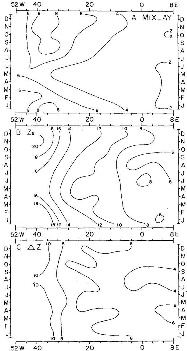
FIG. 7. Longitudinal and annual variation of subsurface thermal structure along profile A (ref. Fig. 1). Quantities are in tens of meters. (a) mixed layer depth MIXLAY; (b) base of thermocline z_b ; (c) thermocline thickness \Delta z .
