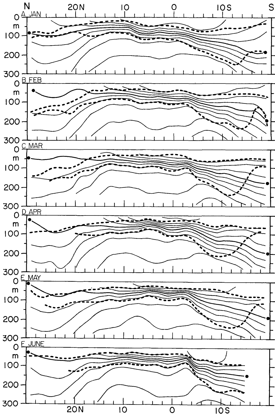
FIG. 10. Monthly meridional cross sections across the Central Atlantic. See Fig. 1 for location of profiles (C-C). Thick solid lines with heavy dots at extremities represent 20°C isotherm and thin solid lines other isotherms at 2°C. Heavy broken lines denote the depth of the mixed layer and the base of the thermocline. Parts A-F: January, February, March, April, May, June.
