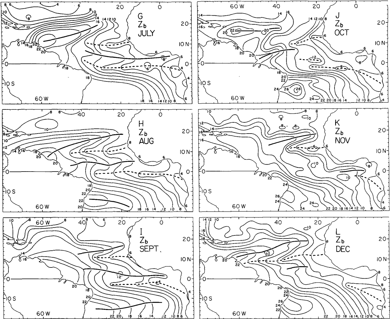
FIG. 3. (Continued). Parts G-L: July, August, September, October, November, December.
