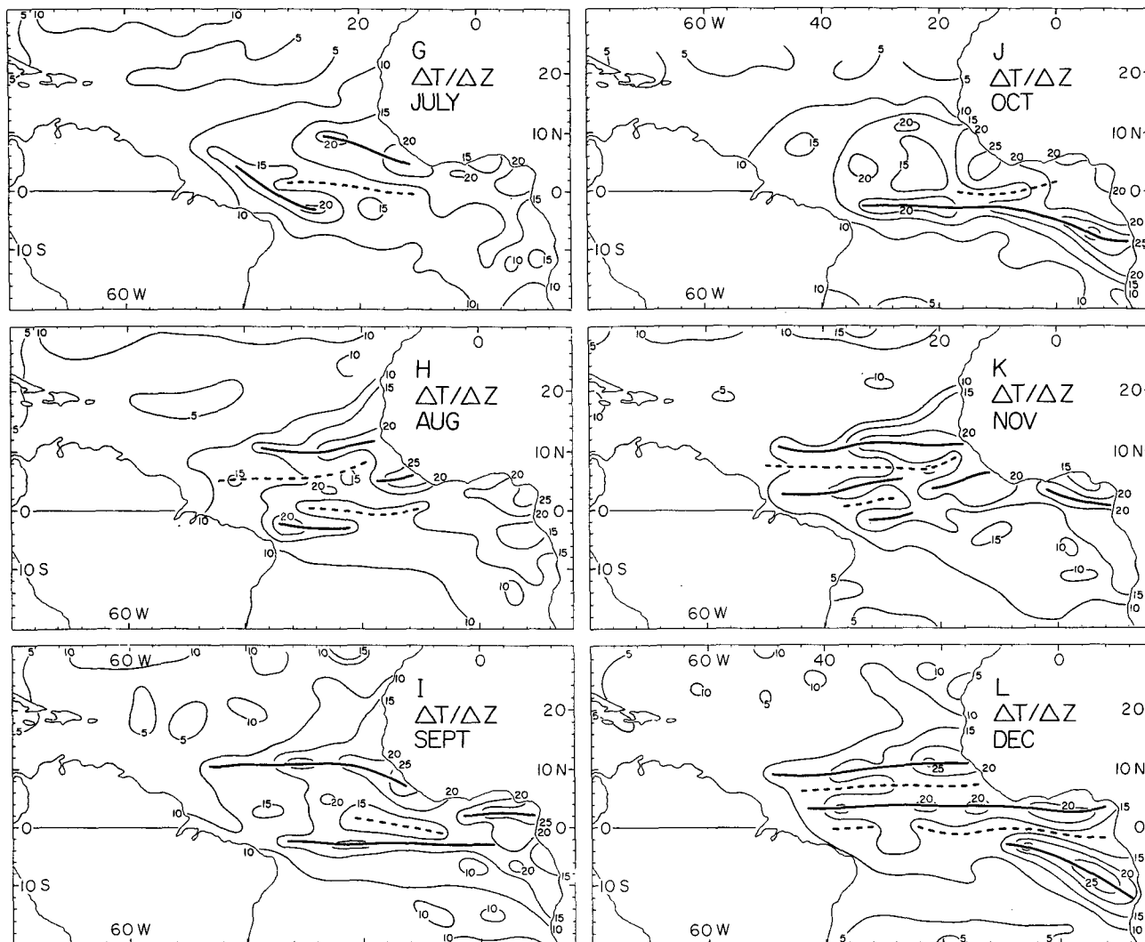
FIG. 5. (Continued). Parts G-L: July, August, September, October, November, December.
