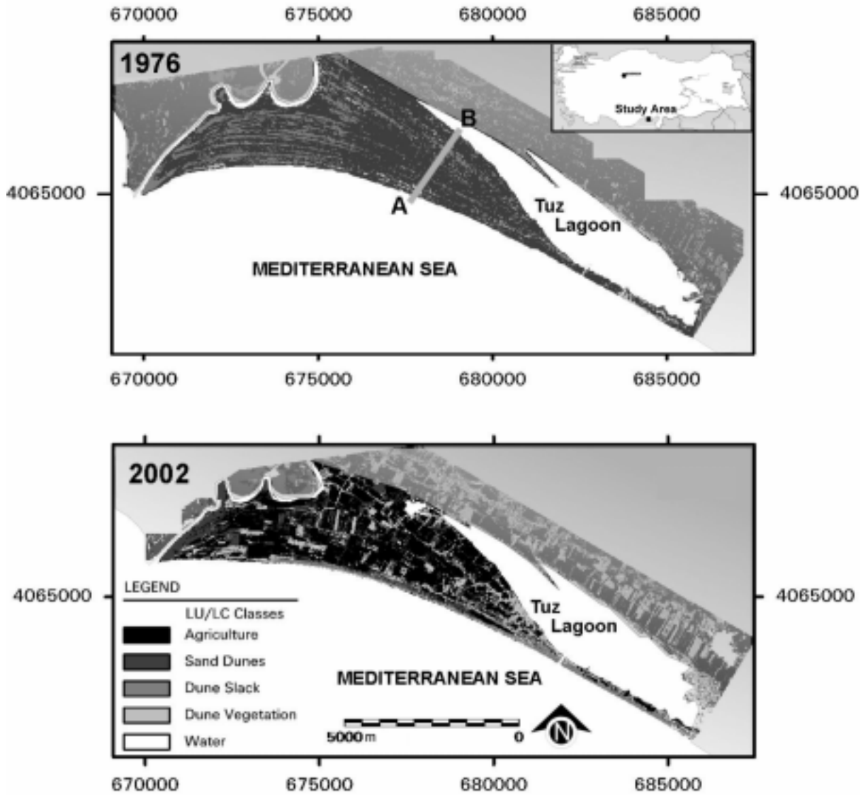
Figure 4. Classified aerial and IKONOS imagery based on spectral data and variogram texture measures.
