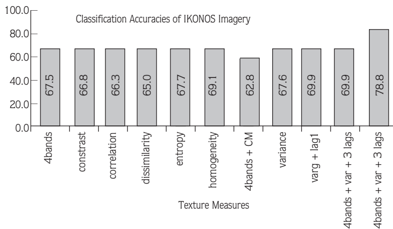
Figure 2. Overall accuracy results of the classifications incorporating texture measures. (CM: Co-occurrence matrix; var: Variance)
