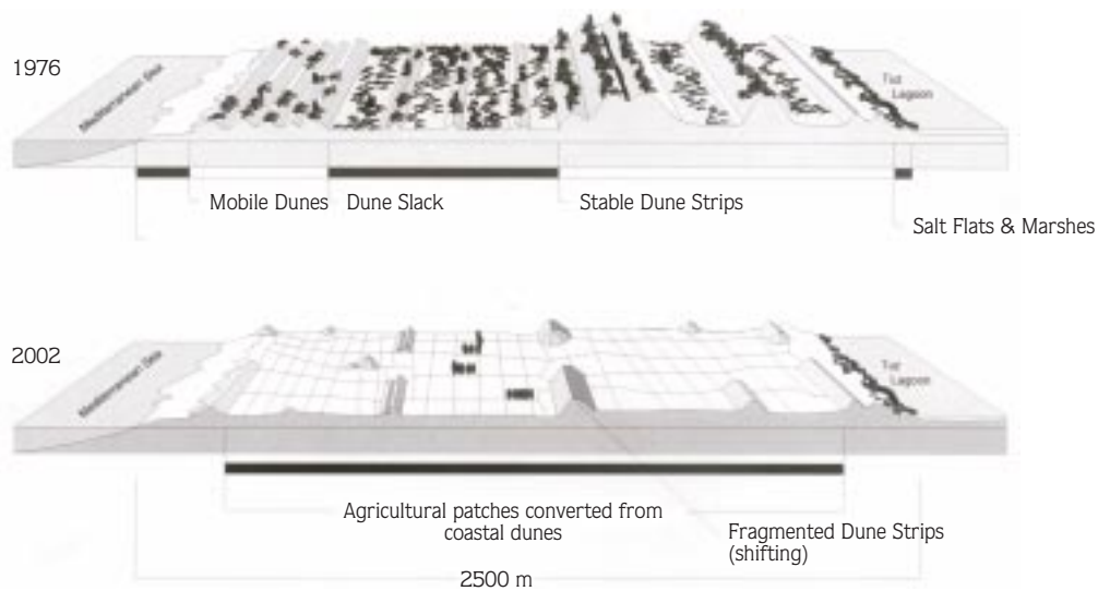
Figure 6. Profiles of the region extracted from classified images (The location is given in Figure 4).
