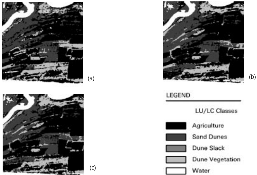
Figure 5. Classifications incorporating various texture measures for parts of the IKONOS imagery (a: variogram lags of 1,2,3 pixels; b: spectral alone; c: homogeneity).
