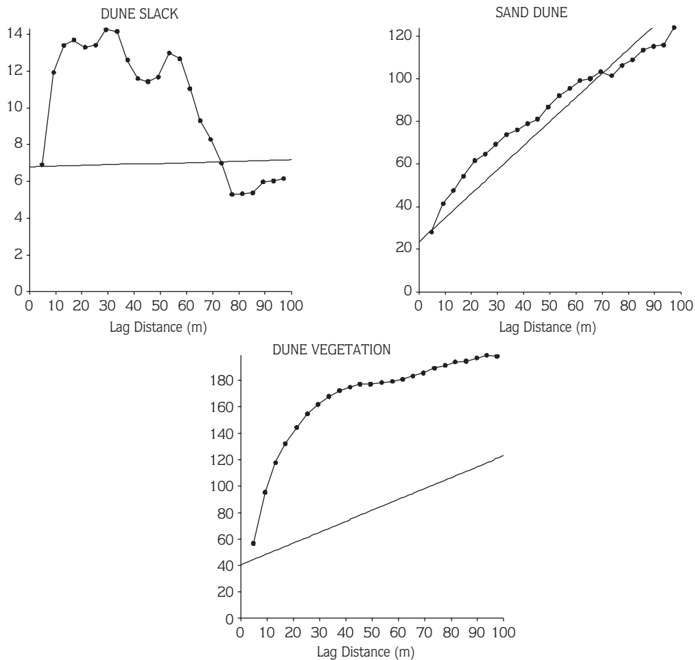
Figure 3. The measured (circles) and modelled (line) variograms from aerial photo image.
