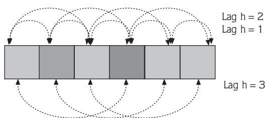
Figure 1. Lags along a transect of pixels. Lags of 1, 2 and 3 pixels are illustrated.
