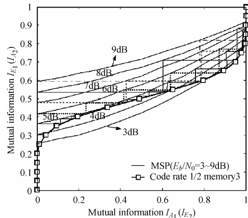
图 2 MSP 映射的迭代译码对应得 EXIT 图解 Fig.2 EXIT chart with MSP mapping and rate 1/2, memory 3 convolutional code
