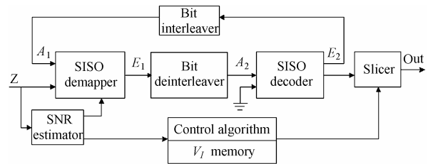
图 3 BICM-ID 系统的迭代控制框图 Fig.3 The diagram of BICM-ID system with iterative control algorithm
