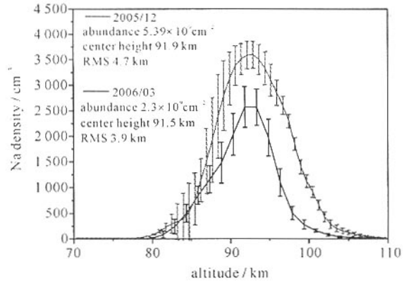
Fig. 3 Monthly average parameters of sodium layer at Dec. 2005 and Mar. 2006 at Hefei
