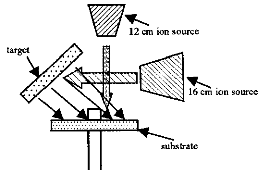
Fig. 4 Dual-ion beam sputtering deposition thin film system
