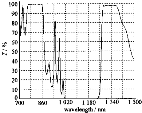
Fig. 2 Theoretical transmittance curve for incident facet on Nd:YAG crystal
