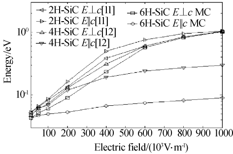
图3 6H-SiC 电子平均能量同电场的关系 Fig. 3 Electron mean energy as a function of the electric field in 6H-SiC at 296 K
