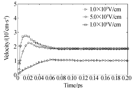
图6 电子横向漂移速度随不同阶跃电场的瞬态变化 Fig. 6 Transient response of electron velocity for E \perp c to different step electric field
