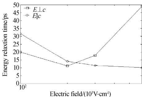
图4 电子能量弛豫时间随电场的变化 Fig. 4 Electron energy relaxation time as a function of the electric field at 296 K
