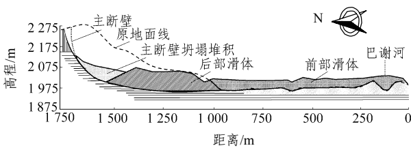
图6 洒勒山滑坡滑后纵剖面 [45] Fig.6 Geological profile of Sale mountain landslide [45]
