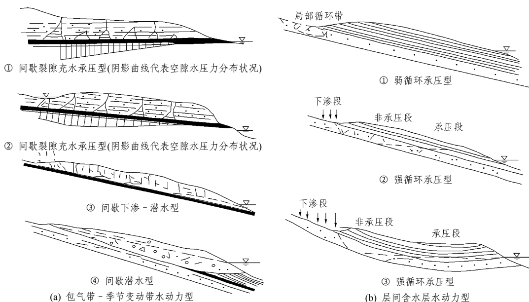
图19 顺向层状体斜坡水动力学基本模型 [45] Fig.19 Hydrodynamics model of consequent rocky slopes [45]
