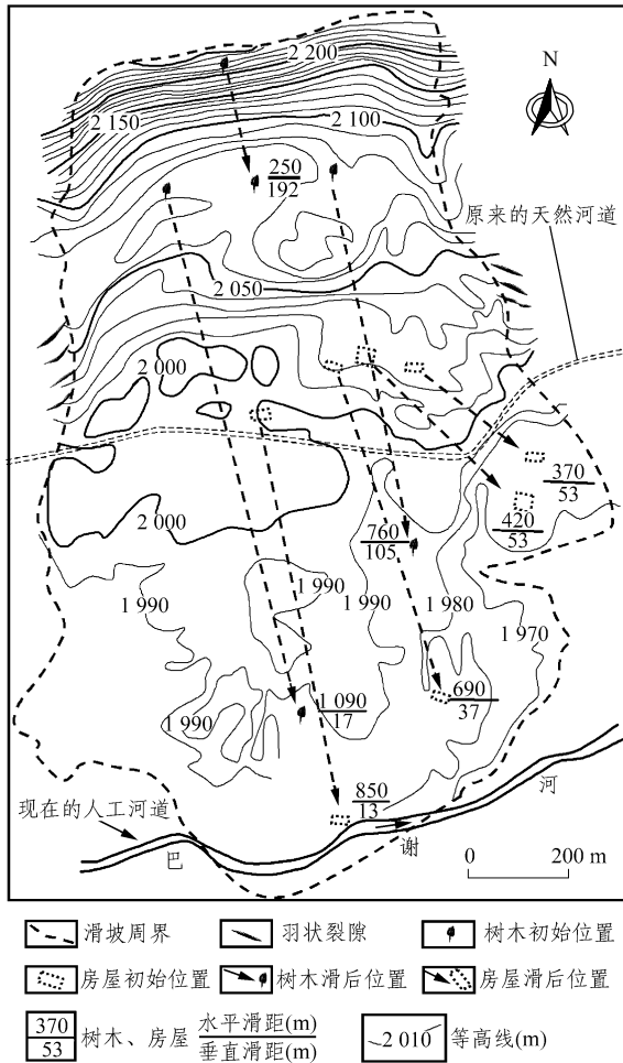
图5 洒勒山滑坡形态平面及滑动矢量图 [44] (略有改动) Fig.5 Plan of Sale mountain landslide and its sliding vector diagram [44] (revised)
