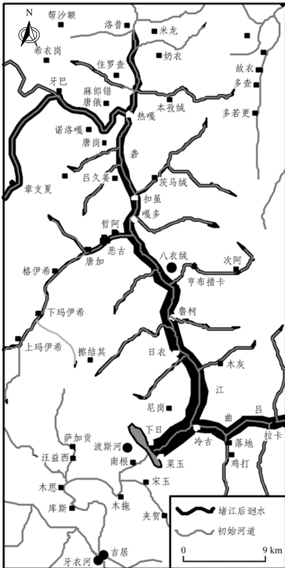
图 2 唐古栋滑坡坝及其回水范围 Fig.2 Tanggudong landslide dam and its backwater scope
