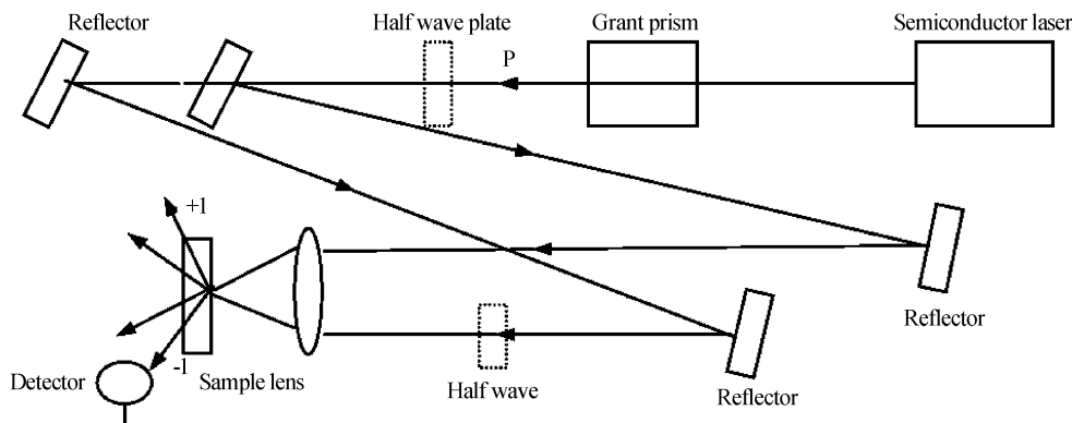
图 2 实验光路图 Fig. 2 The sketch of the equipment
