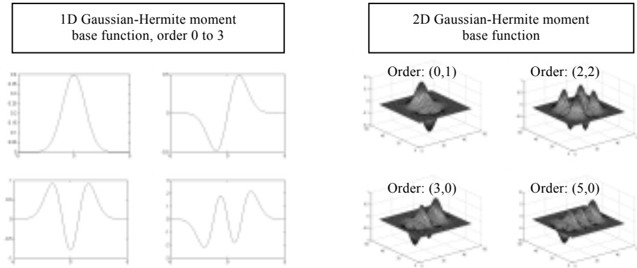
Fig.2 Spatial behavior of Gaussian-Hermite moments base functions
