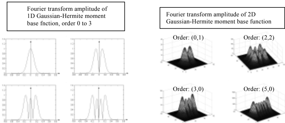
Fig.3 Frequency domain behavior of Gaussian-Hermite moments base functions
