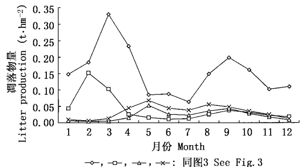
图4 主要优势种叶凋落节律 Fig.4 Seasonal rhythm of leaf litter of dominant species
