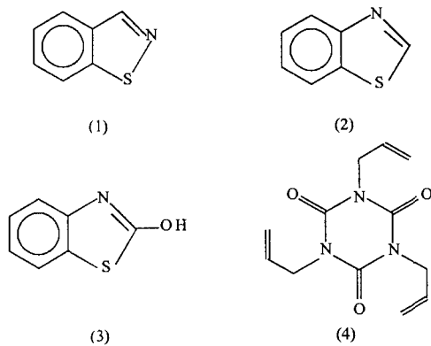
图3 PI312777 土培的根系分泌物乙醚萃取物中杂环类化合物结构 Fig.3 Heterocycle of ether extracts from the PI312777 root exudates grown in soil.
