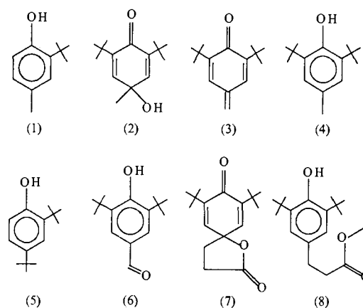
图 2 PI312777 土培的根系分泌物乙醚萃取物中酚醌类化合物结构 Fig.2 Phenols or quinones of ether extracts from the PI312777 root exudates grown in soil.
