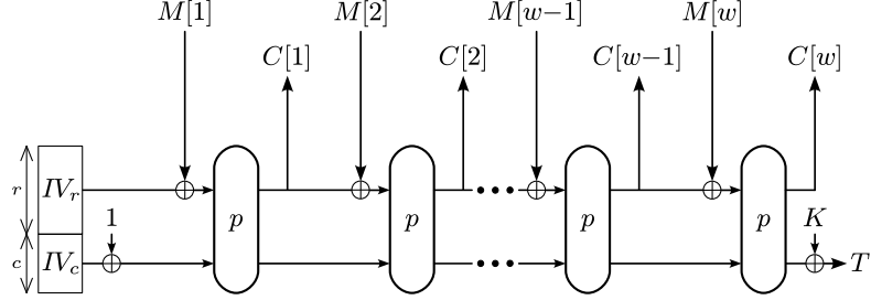
Fig. 1. The APE mode of operation (encryption). If there is no associated data ( A = \emptyset ), we set IV_r := 0 and IV_c := K . Otherwise, IV is computed from the associated data (see Fig. 2).
