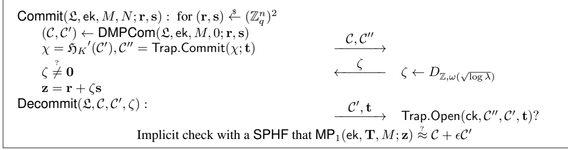
Figure 3: DMPCom' Commitment Scheme for SPHF
