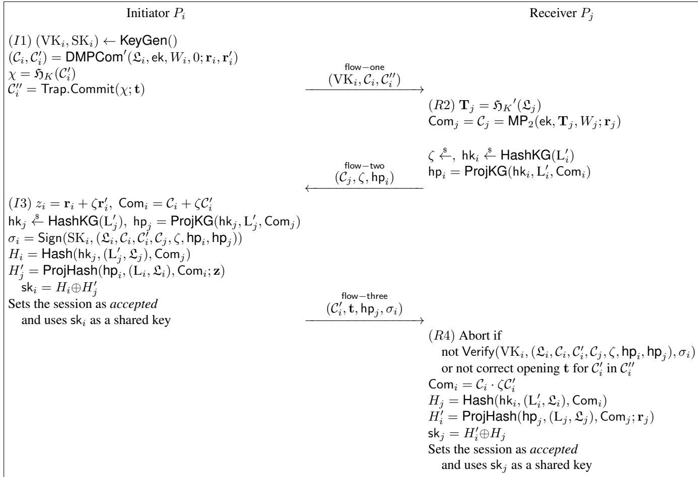
Figure 11: Description of the password-authenticated key-exchange protocol for players (P_i, \text{ssid}) , with index i , password W_i , random tape \omega_i , label \mathcal{L}_i = (\mathcal{L}, \text{VK}_i) , languages \mathcal{L}_i = \mathcal{L}'_i = \{W_i\} and (P_j, \text{ssid}) , with index j , password W_j , random tape \omega_j , label \mathcal{L}_j = \mathcal{L} , languages \mathcal{L}_j = \mathcal{L}'_j = \{W_j\} . The label is \mathcal{L} = (\text{sid}, \text{ssid}, P_i, P_j) . The random values used in the commitments (witnesses) are all included in (\mathbf{r}_i, \mathbf{r}'_i) and \mathbf{r}_j .
