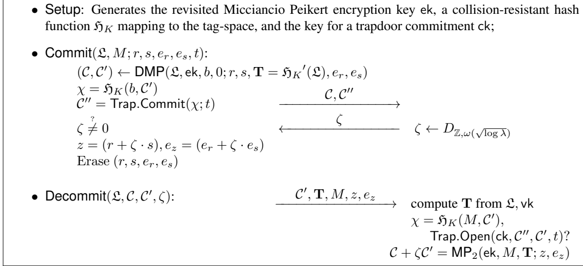
Figure 8: DMP Commitment Scheme
