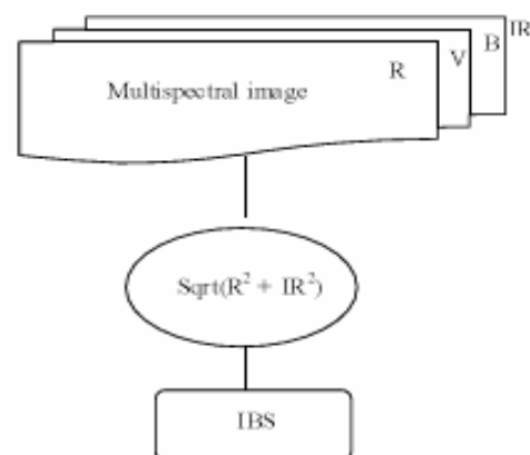
Figure 3.3. Computation of soil index
