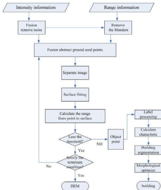
Figure 1. Process frame
