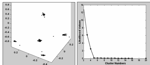
Figure 5. Plot of the direction cosines for each planar patch (a, left) and the elbow-joint graph (b, right).
