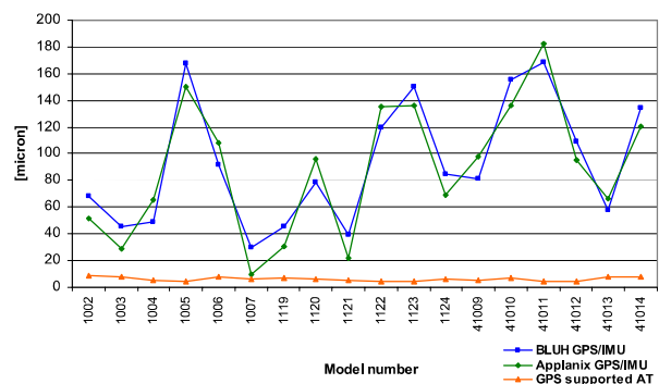
Figure 7. Comparison of the y parallaxes
