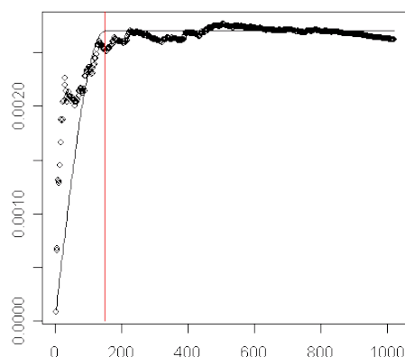
Figure 2: Estimation of the optimal neighborhood size: A spherical variogram function is fitted to the variance-neighborhood plot to estimate the range
