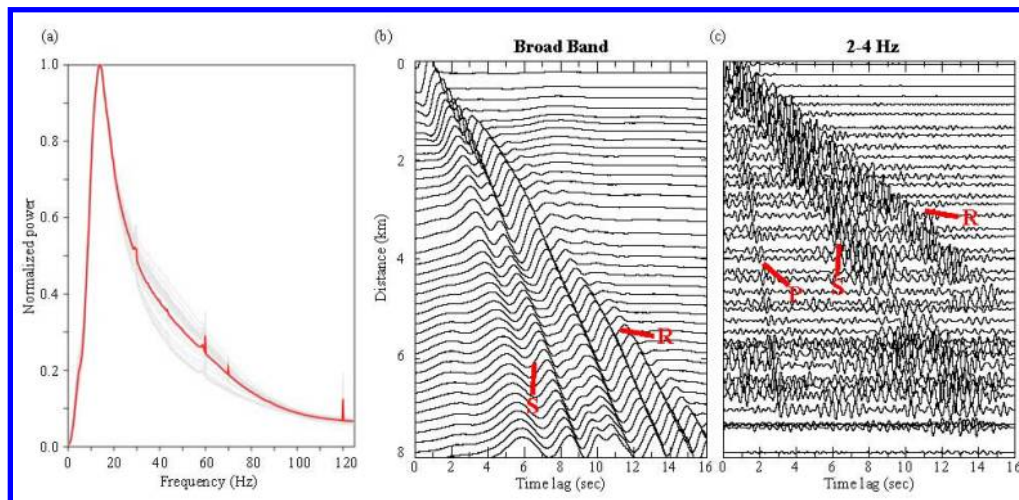
Figure 2. (a) Average spectrum of all receivers averaged over one day. The light gray lines show hourly variations. (b) Broad-band stacked cross-correlation record section. (c) 2-4 Hz bandpass-filtered cross-correlation record section.
