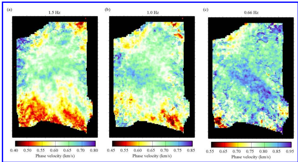
Figure 5. Rayleigh wave phase velocity maps at 1.5 Hz, 1.0 Hz, and 0.66 Hz.
