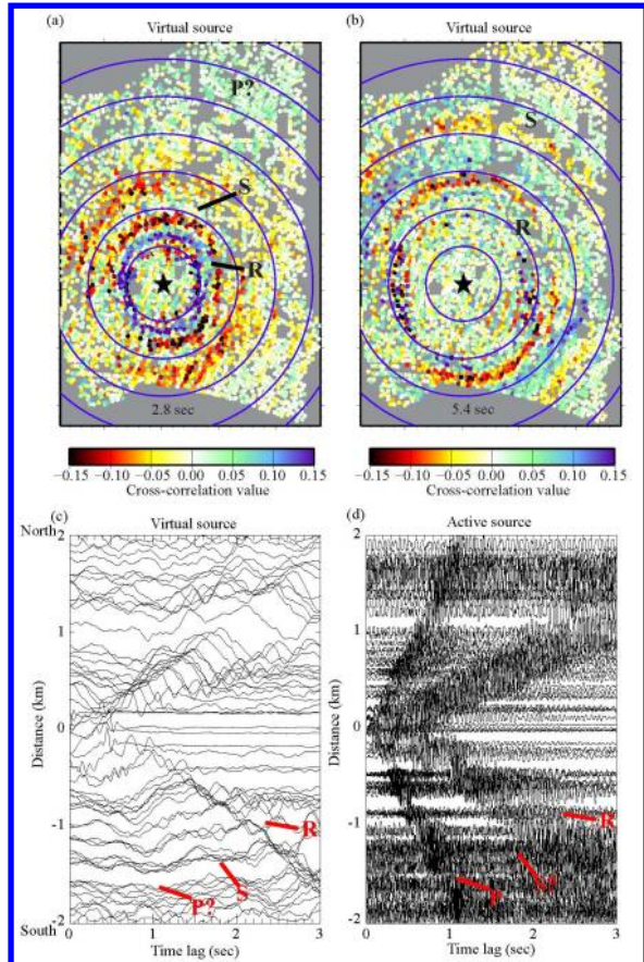
Figure 3. (a)-(b) Time slices of a virtual source. Contour interval is 1 km. (c)-(d) Comparison of virtual source and vibrator source.
