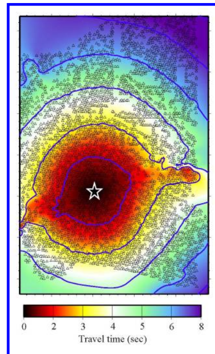
Figure 4. Rayleigh wave phase travel time surface. The contours are 1.5-sec travel time intervals. The phase velocity can be estimated by the gradient of this surface.
