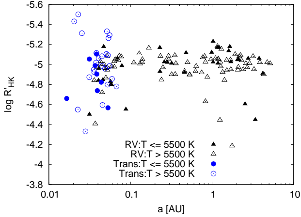
Fig. 5. Dependence of the activity index \log R'_{\text{HK}} on the semi-major axis. Triangles are exoplanetary systems discovered by RV technique, circles are systems discovered by transit method.
