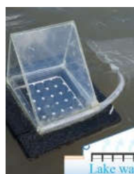
A floating solar still prototype that researchers used for some of experiments. Credit: University at Buffalo.
