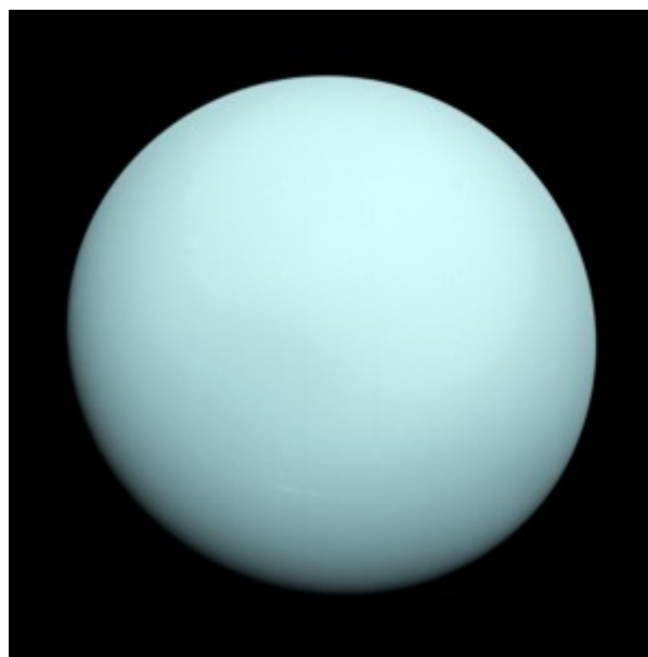
Uranus (NASA/JPL-Caltech)
