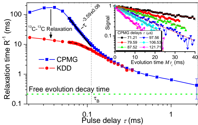
Figure 1: (Color online) Experimental relaxation times of the probe spin under the application of CPMG (squares) and KDD (circles) sequences. The black solid line represents a power law fitting to the CPMG data and the green dotted line the asymptotic free evolution decay rate. The black dashed line is a fitting to the KDD data with an expression (R_{13C} + C'\tau^\alpha)^{-1} . Inset: Experimental signal decays of the probe spin as a function of the evolution time under CPMG dynamical decoupling. Different curves correspond to different pulse delays. The straight lines represent exponential fits.
