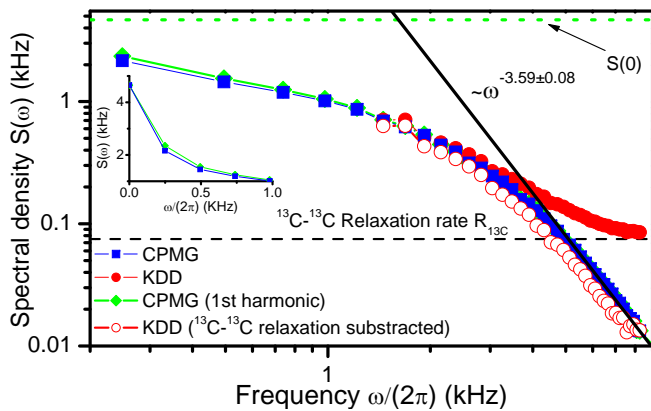
Figure 2: (Color online) Experimentally determined noise spectral density. The inset shows in a linear scale the low frequency regime. The green dotted line represents the free evolution decay rate of the probe spin, i.e. S(0) .
