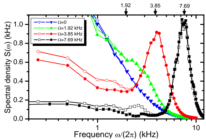
Figure 3: (Color online) Experimentally determined noise spectral density for a modulated system-environment interaction. The empty symbols were obtained when only the first harmonic is considered, the full symbols show the results from the exact method.
