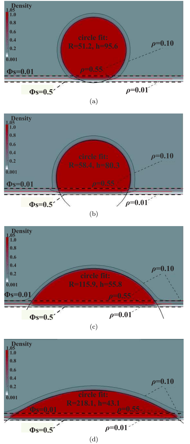
FIG. 6. Sessile circular droplet at equilibrium. The equilibrium contact angle \theta_Y = \arccos(1 - h/R) is computed via circle fitting (solid black line); R is the circle radius, and h indicates the droplet height (measured from the outer boundary of the simulation domain). Contour lines (solid) for the fluid density, \rho = 0.01, 0.1, 0.55 , indicate a gradual growth of the interfacial film thickness as the attraction parameter G_A increases. Contour lines (dashed) for the solid probability function, \rho_w = 0.1, 0.5 , contain the interfacial region where a disjoining pressure is active. All cases correspond to G_R = 1.33 and R_0 = 50 . (a) G_A = 0.0 , \theta_Y = 150^\circ . (b) G_A = 0.2 , \theta_Y = 112^\circ . (c) G_A = 0.5 , \theta_Y = 58.7^\circ . (d) G_A = 0.7 , \theta_Y = 36.7^\circ .
