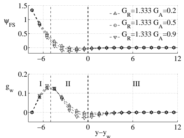
FIG. 3. Fluid-solid potential (Top panel), \psi_{FS} , and volumetric force (Bottom panel), g_w , for interaction parameters within the range employed in simulations: G_R = 1.33 ; G_A = 0.2, 0.5 , and 0.9 . The lines in the plots are interpolation curves fitting the computed node values [see Appendix]. The y -axis is in the direction normal to a wall ( y coordinates are indicated in lattice units). The hydrodynamic region (I) begins at y_w \simeq 8.5 where \phi_S(y_w) = 0.01 (the opposite boundary is located at y_w = L_y - 7.5 ). The normal component g_w (given in lattice units) gives rise to a disjoining pressure \Pi = -\rho g_w that dominates within the interfacial region (II).
