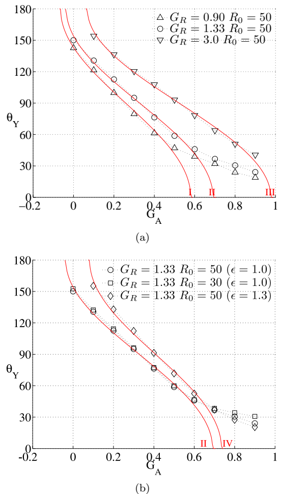
FIG. 8. Equilibrium contact angle \theta_Y for a two-dimensional droplet on a flat surface versus attraction parameter G_A . The reference radius R_0 determines the droplet volume (per unit width) V_d = \pi R_0^2 . The same equilibrium contact angle can be obtained using infinite combinations of wall interaction parameters G_R and G_A . Solid lines are estimations by an augmented Young-Laplace equation \cos \theta_Y \approx (E_0 + k_A G_A)/\gamma : (I) E_0 = -0.64 , k_A = 2.5 ; (II) E_0 = -0.87 , k_A = 2.2 ; (III) E_0 = -1.92 , k_A = 1.76 ; (IV) E_0 = -1.0 , k_A = 3.06 ; in all cases \gamma = 0.09 . Deviations from a linear approximation for the surface energy excess \Delta E = k_A G_A are observed for \theta_Y < 45^\circ .
