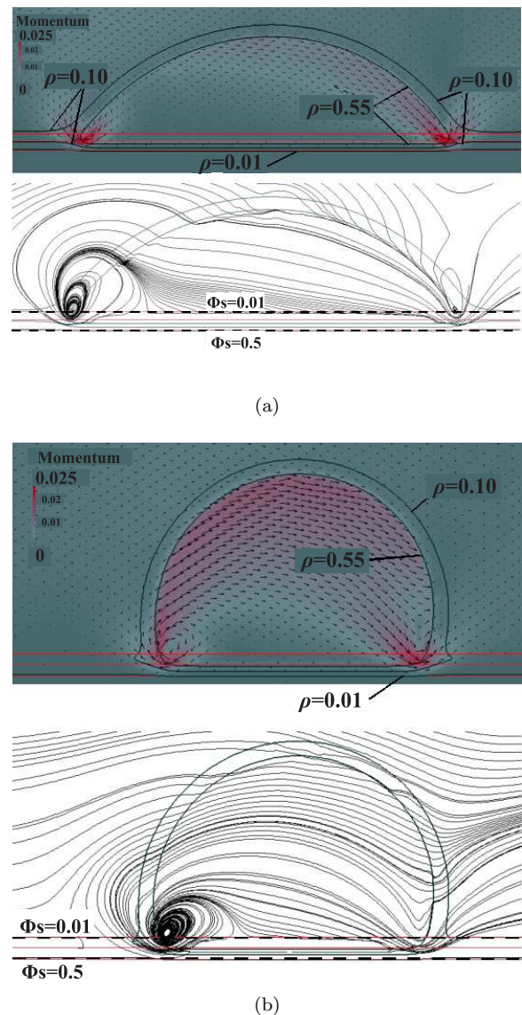
FIG. 11. Fluid momentum magnitude |\mathbf{M}^{(1)}| (top panels in the subfigures) and velocity streamlines (bottom panel in the subfigures) for droplet motion under pressure-driven flow. (a) Static contact angle \theta_Y = 58^\circ ( G_R = 1.33 , G_A = 0.5 , \epsilon = 1.0 ). (b) Static contact angle \theta_Y = 113^\circ ( G_R = 1.33 , G_A = 0.2 , \epsilon = 1.0 )
