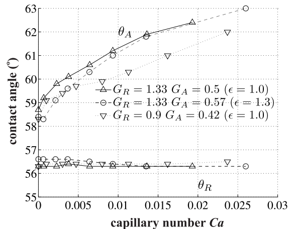
FIG. 10. Advancing and receding contact angles versus capillary number Ca = U\mu_L/\gamma (for the definition of the appropriate U see text). All sets of interaction parameters result in the same value for the equilibrium angle \theta_Y \simeq 58^\circ but different contact angle dynamics. The functional form of the disjoining pressure produces a finite static hysteresis of the contact angles.
