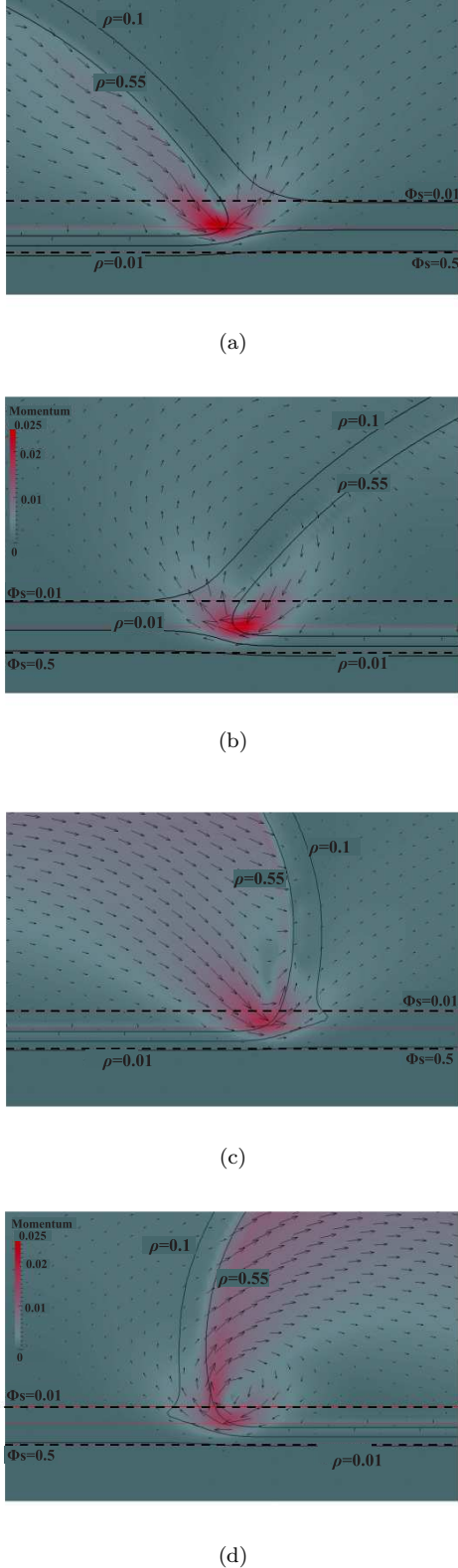
FIG. 12. Flow patterns in the vicinity of the advancing and receding contact lines observed on a hydrophilic surface and on a hydrophobic surface. (a) Advancing contact line, static contact angle \theta_Y = 58^\circ ( G_R = 1.33 , G_A = 0.5 , \epsilon = 1.0 ). (b) Receding contact line, static contact angle \theta_Y = 58^\circ ( G_R = 1.33 , G_A = 0.5 , \epsilon = 1.0 ). (c) Advancing contact line, static contact angle \theta_Y = 113^\circ ( G_R = 1.33 , G_A = 0.2 , \epsilon = 1.0 ). (d) Receding contact line, static contact angle \theta_Y = 113^\circ ( G_R = 1.33 , G_A = 0.2 , \epsilon = 1.0 ).
