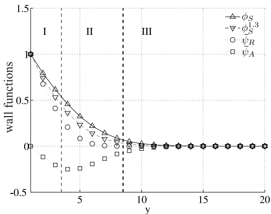
FIG. 2. Wall functions determined before dynamic simulation: wall probability \phi_S^\epsilon ( \epsilon = 1, 1.3 ); repulsive and attractive components of \psi_{FS} = G_R\psi_R + G_A\psi_A ; y (in lattice units) is in the direction normal to a wall (bottom or top). The lines in the plots are interpolation curves fitting the computed node values [see Appendix]. The value of the wall probability is used to determine three regions: (I) solid substrate ( \phi_S > 0.5 ) where short-range (fluid-solid) interactions are dominant; (II) interfacial boundary layer ( 0.5 \leq \phi_S \leq 0.01 ) where surface forces are significant; (III) hydrodynamic region or fluid bulk ( \phi_S < 0.01 ) where surface forces become negligible.
