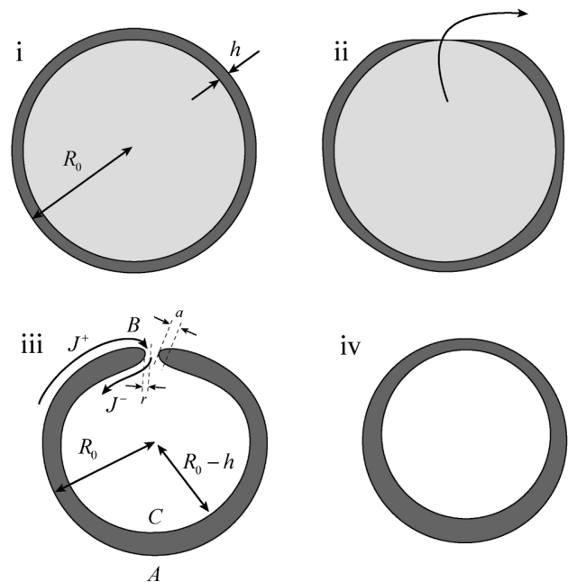
Fig. 1 Stages in the surface-diffusion driven formation of hollow nanoparticles. (i) A core-shell nanoparticle of radius R_0 and shell thickness h ; (ii) shape fluctuations in the outer surface expose the core, allowing it to be dissolved away; (iii) a pinhole of radius r exists in the shell, but quickly closes up because of a diffusional flux from the convex outer surface A through the pinhole edge B and into the inner concave surface C . (iv) When the radius of curvature of the pinhole edge a becomes sufficiently large, the net flux at the pinhole edge J^+ - J^- is positive, closing the pinhole and leaving a hollow nanoparticle.
