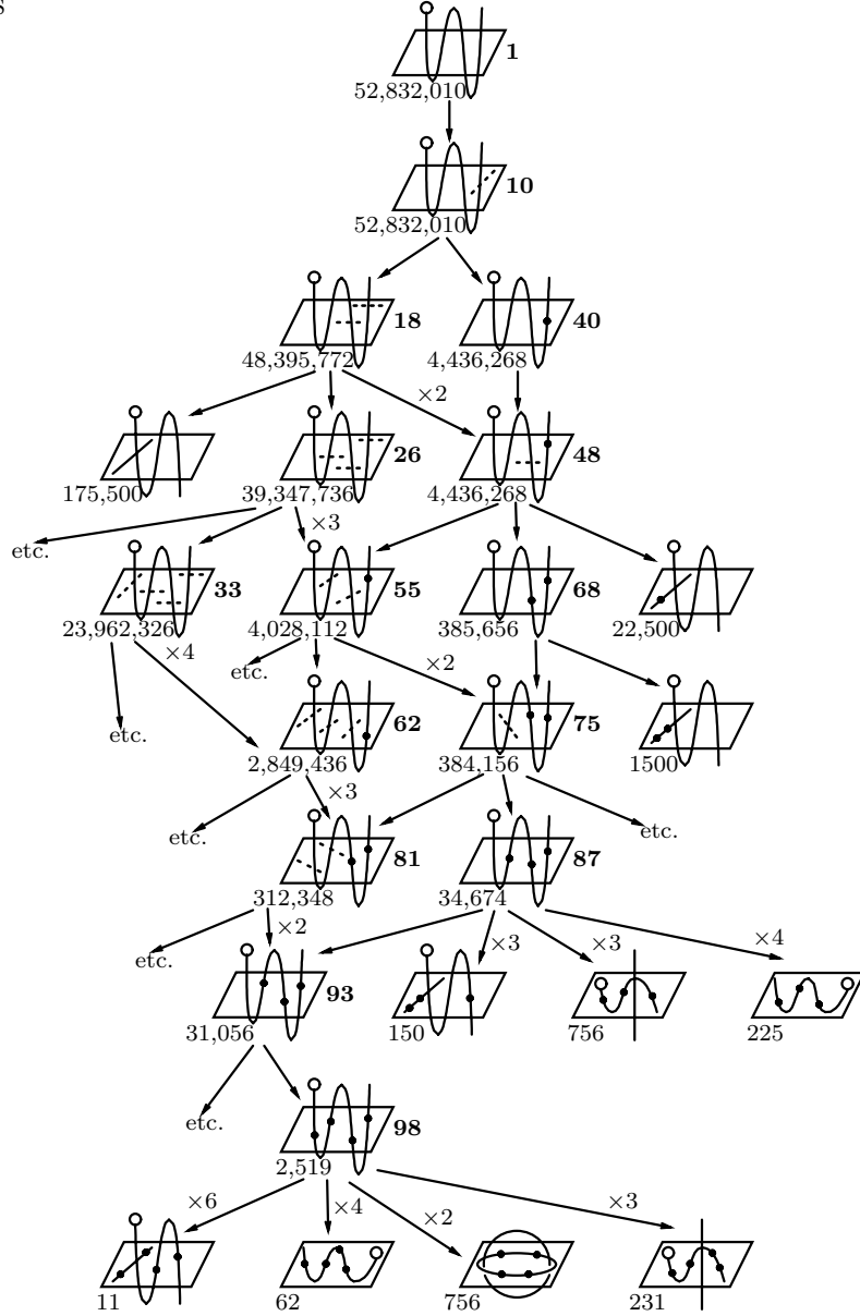
FIGURE 12. Counting quartic elliptic space curves through 16 general lines
