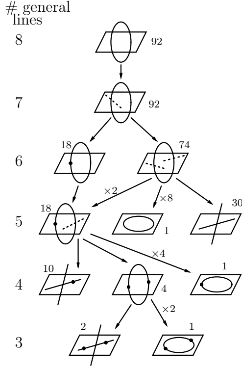
FIGURE 2. Counting 92 conics in \mathbb{P}^3 through 8 general lines
